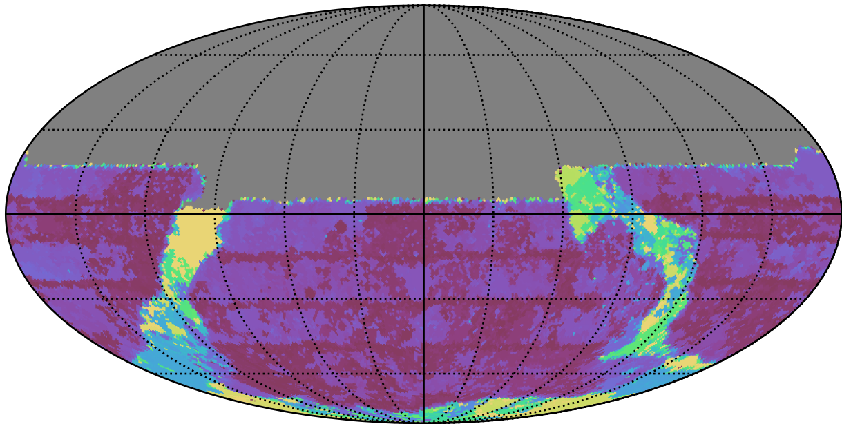
too_100_1v3.4_10yrs All sky u band: Max Inter-Night Gap
