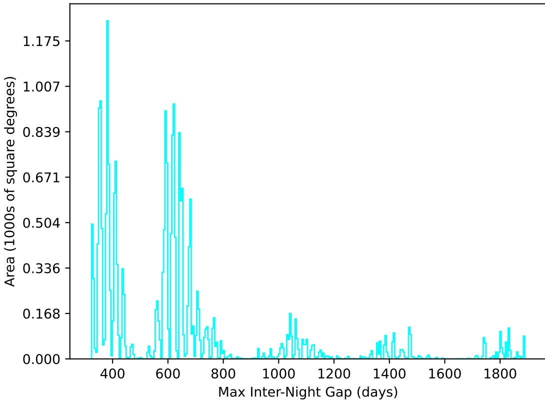
too_100_1v3.4_10yrs All sky u band: Max Inter-Night Gap
