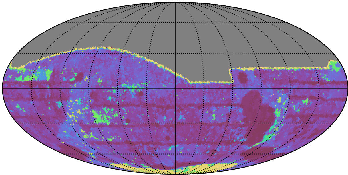
too_100_1v3.4_10yrs All sky i band: Max Inter-Night Gap
