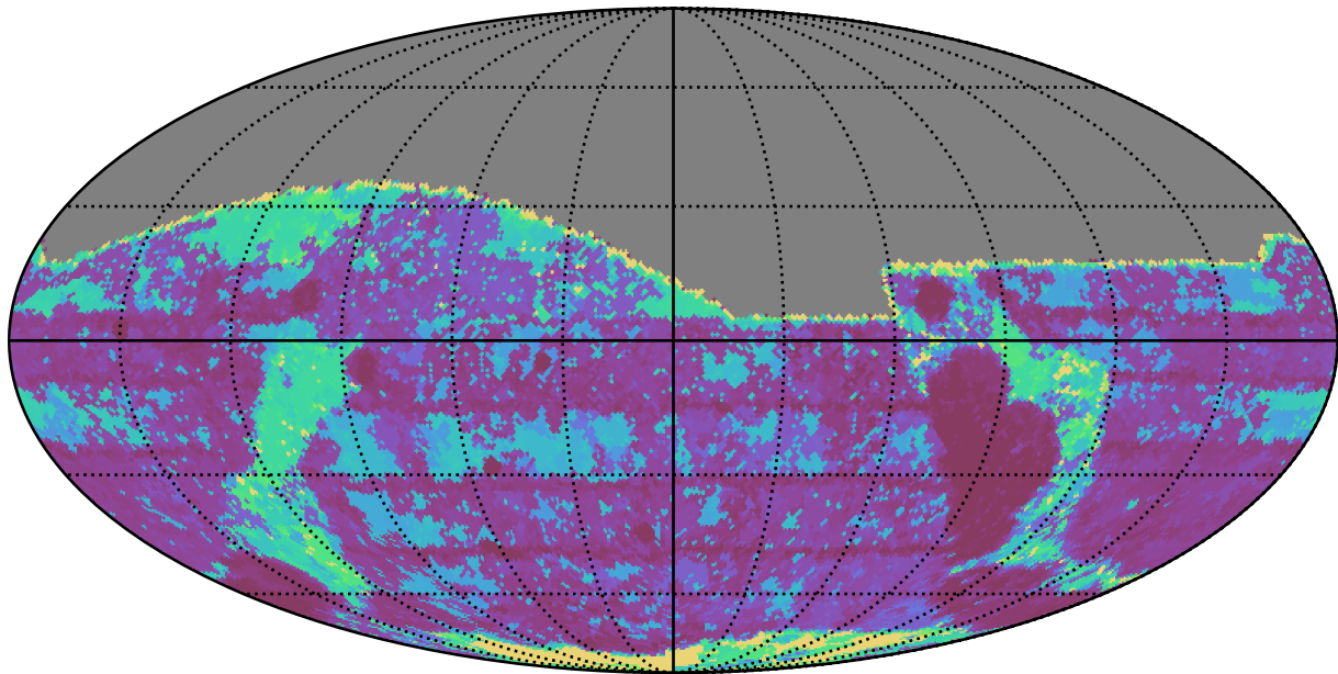
too_100_1v3.4_10yrs All sky g band: Max Inter-Night Gap
