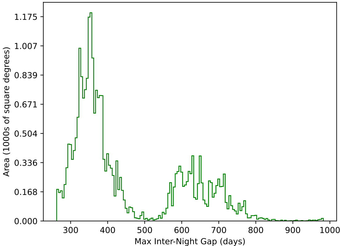
too_100_1v3.4_10yrs All sky g band: Max Inter-Night Gap
