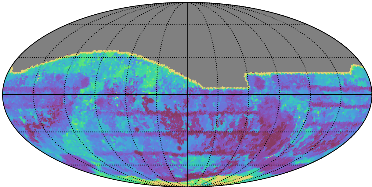
too_100_1v3.4_10yrs All sky all bands: Max Inter-Night Gap
