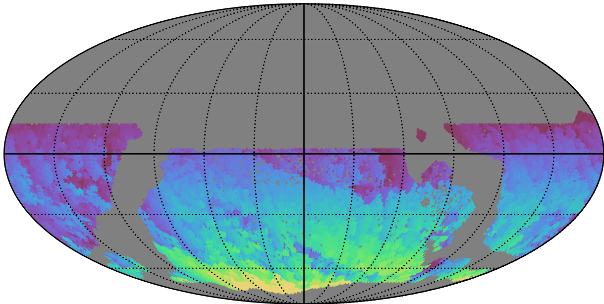
too_100_1v3.4_10yrs WFD z band: Max HA
