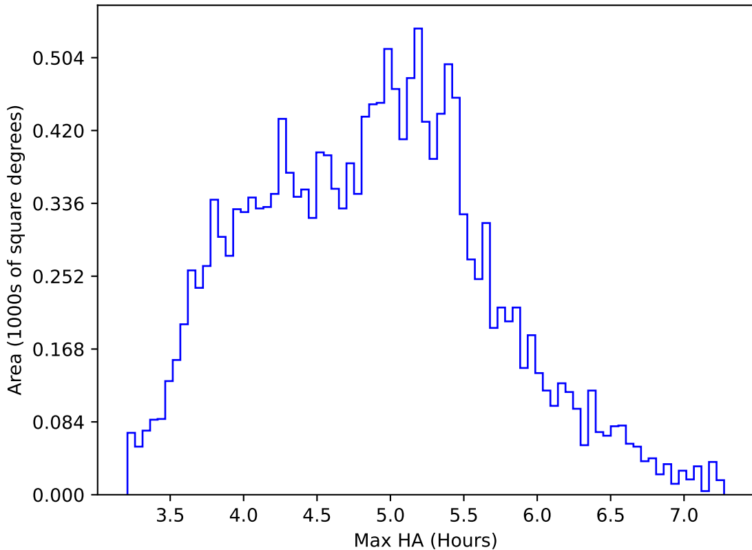
too_100_1v3.4_10yrs WFD z band: Max HA
