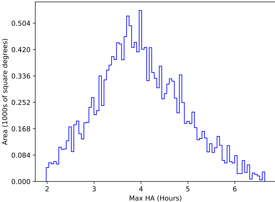
too_100_1v3.4_10yrs WFD u band: Max HA
