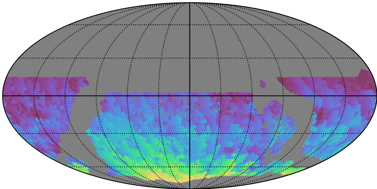
too_100_1v3.4_10yrs WFD r band: Max HA
