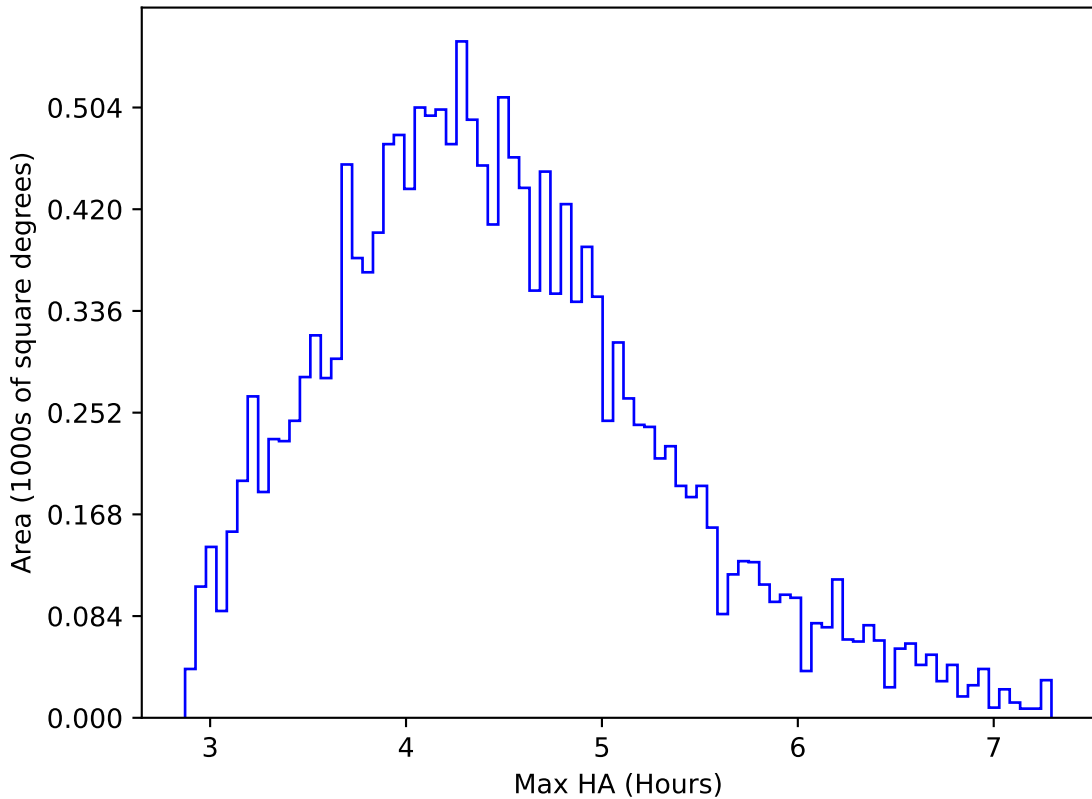
too_100_1v3.4_10yrs WFD r band: Max HA
