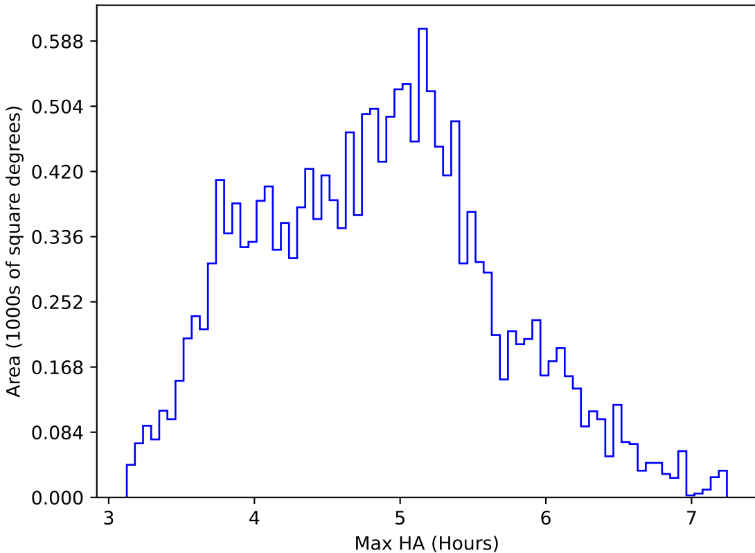
too_100_1v3.4_10yrs WFD i band: Max HA
