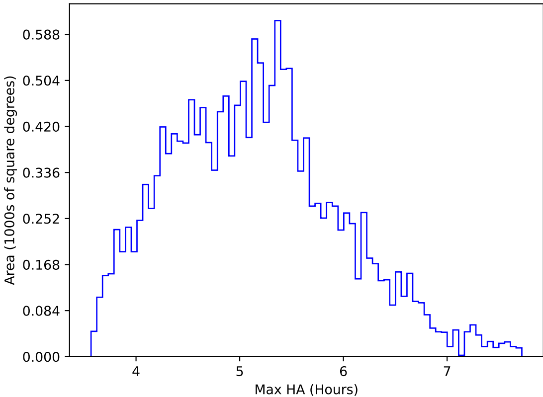
too_100_1v3.4_10yrs WFD all bands: Max HA
