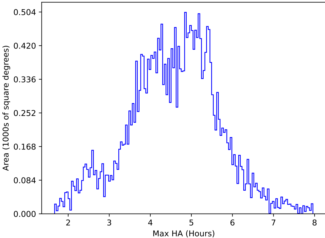
too_100_1v3.4_10yrs All sky z band: Max HA
