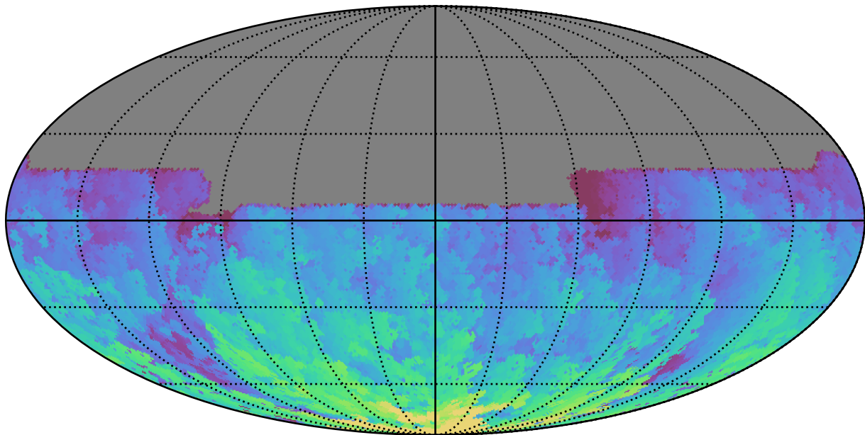
too_100_1v3.4_10yrs All sky u band: Max HA
