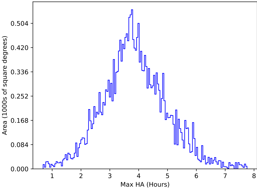
too_100_1v3.4_10yrs All sky u band: Max HA
