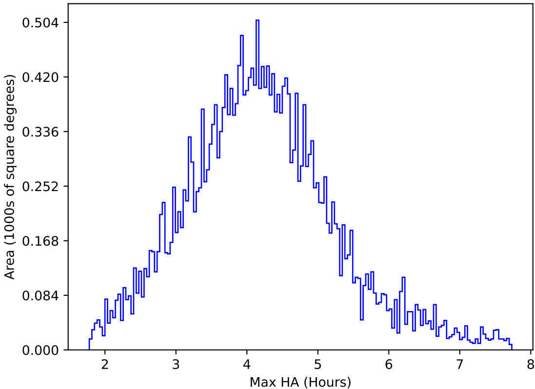
too_100_1v3.4_10yrs All sky r band: Max HA
