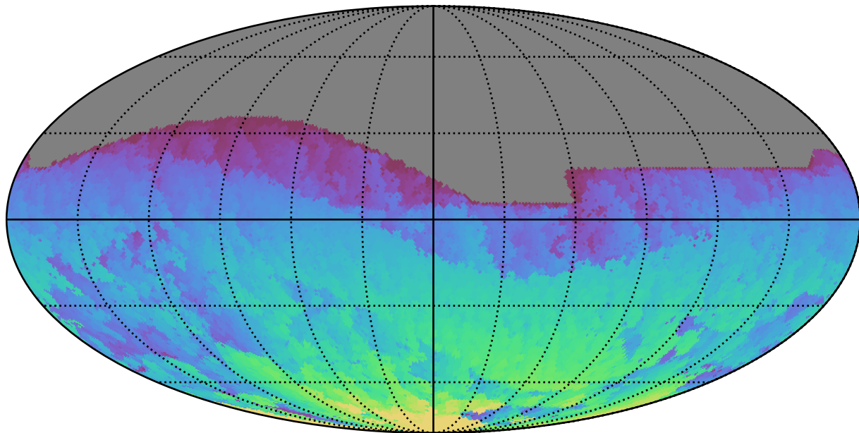
too_100_1v3.4_10yrs All sky i band: Max HA
