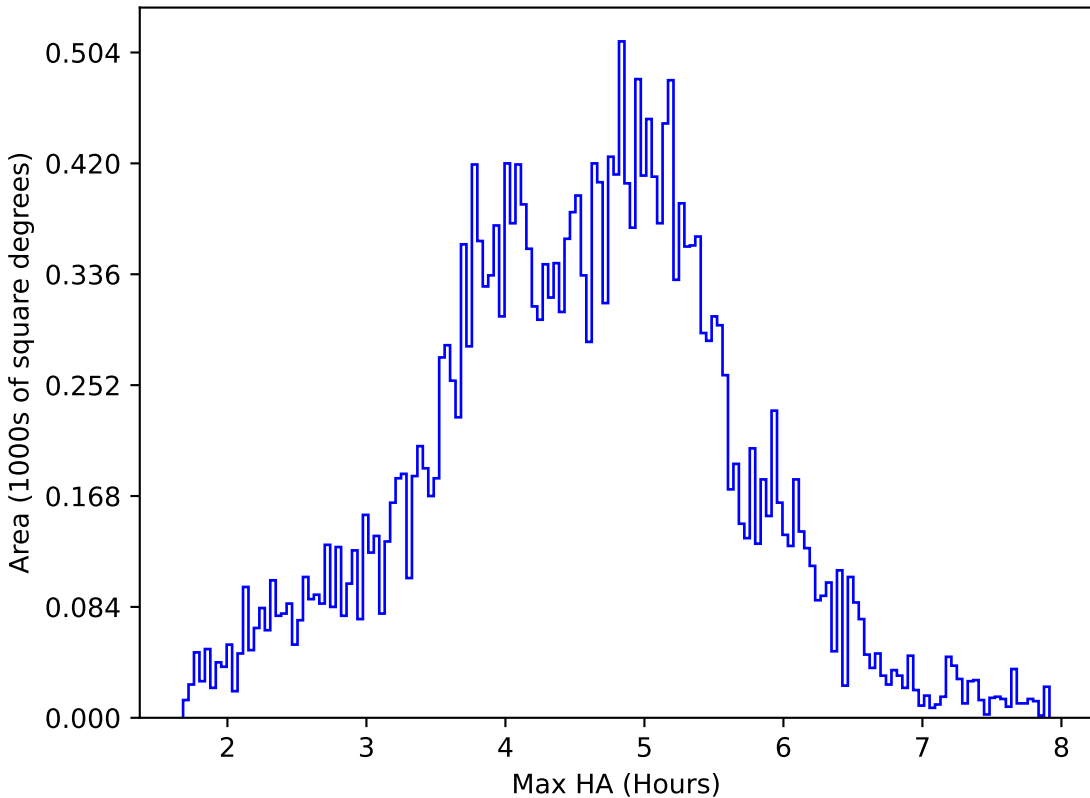
too_100_1v3.4_10yrs All sky i band: Max HA
