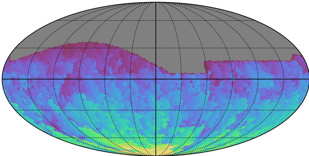
too_100_1v3.4_10yrs All sky g band: Max HA
