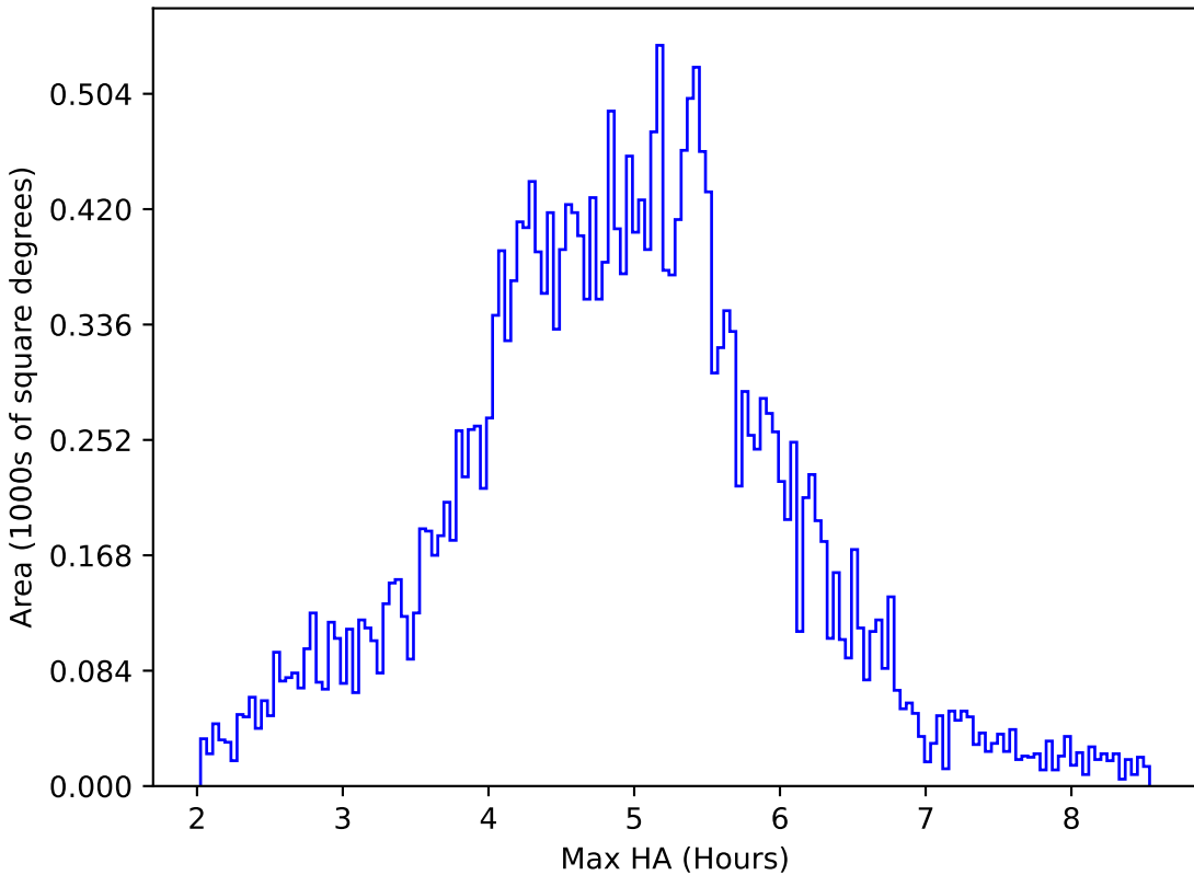
too_100_1v3.4_10yrs All sky all bands: Max HA
