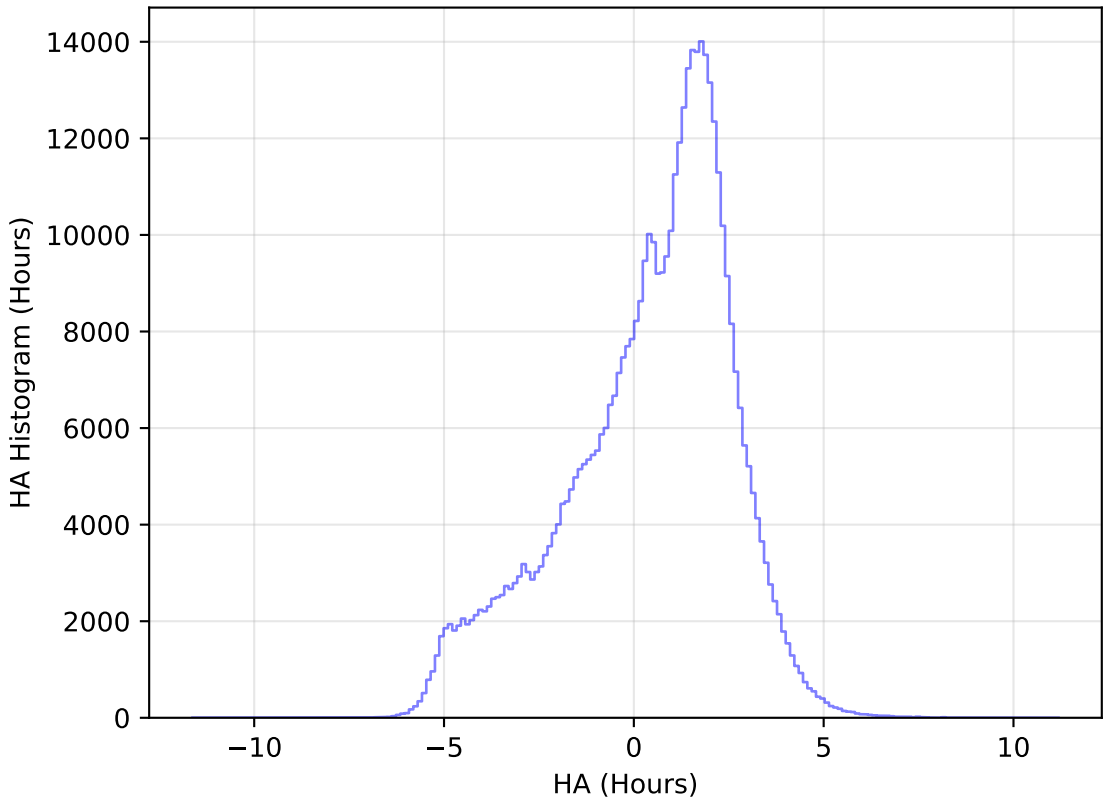
too_100_1v3.4_10yrs WFD r band: HA Histogram
