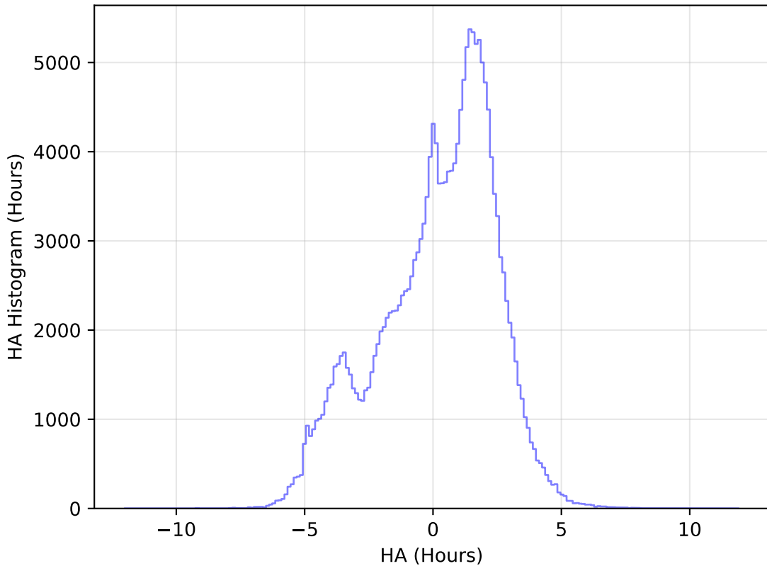
too_100_1v3.4_10yrs WFD g band: HA Histogram
