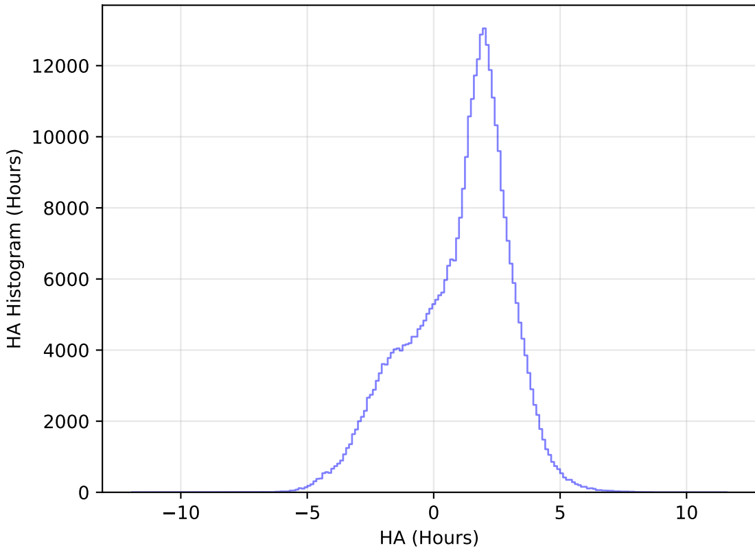
too_100_1v3.4_10yrs All sky y band: HA Histogram
