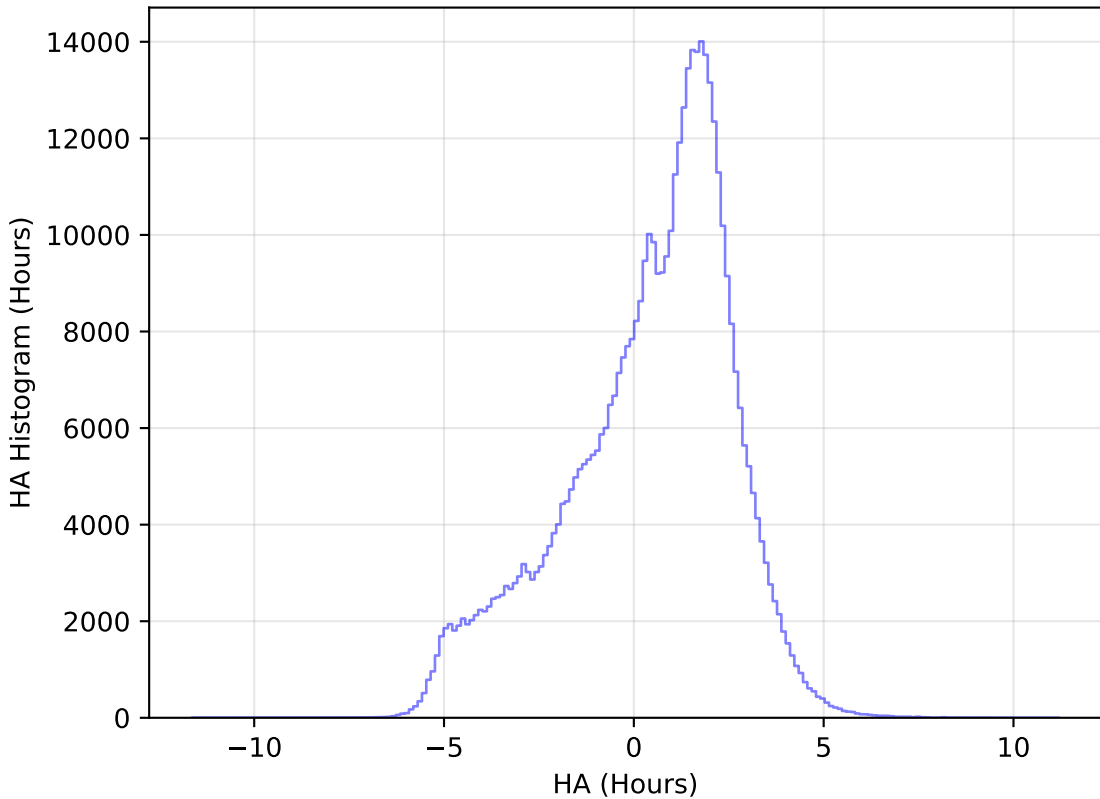
too_100_1v3.4_10yrs All sky r band: HA Histogram
