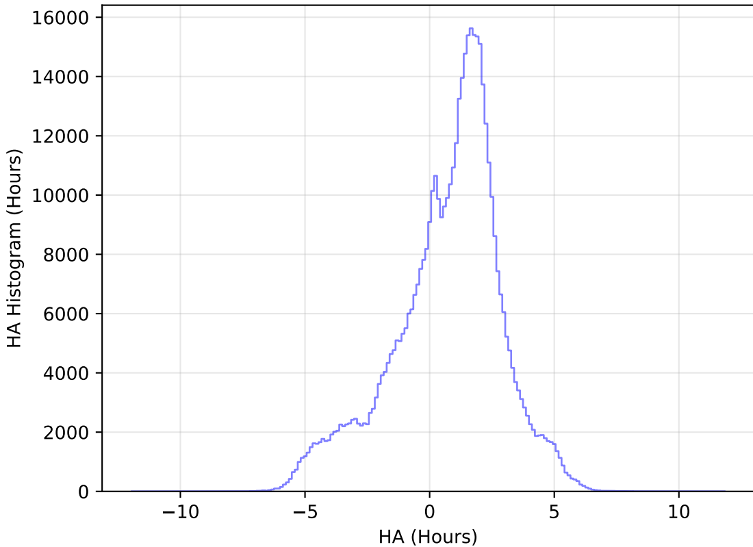
too_100_1v3.4_10yrs All sky i band: HA Histogram
