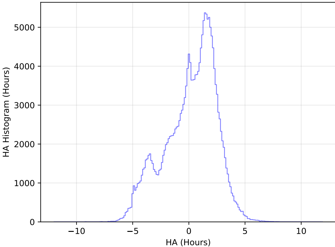
too_100_1v3.4_10yrs All sky g band: HA Histogram
