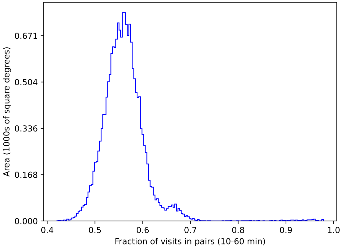
too_100_1v3.4_10yrs gri WFD: Fraction of visits in pairs (10-60 min)
