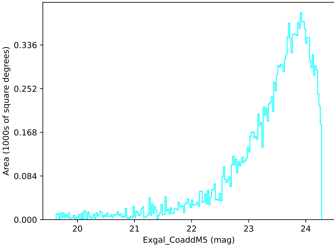
too_100_1v3.4_10yrs Yr 3-4 u band: Exgal_CoaddM5
