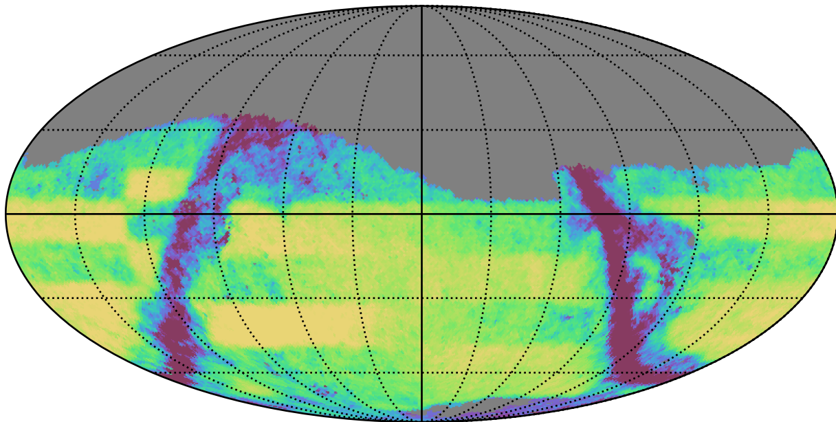
too_100_1v3.4_10yrs Yr 3-4 r band: Exgal_CoaddM5
