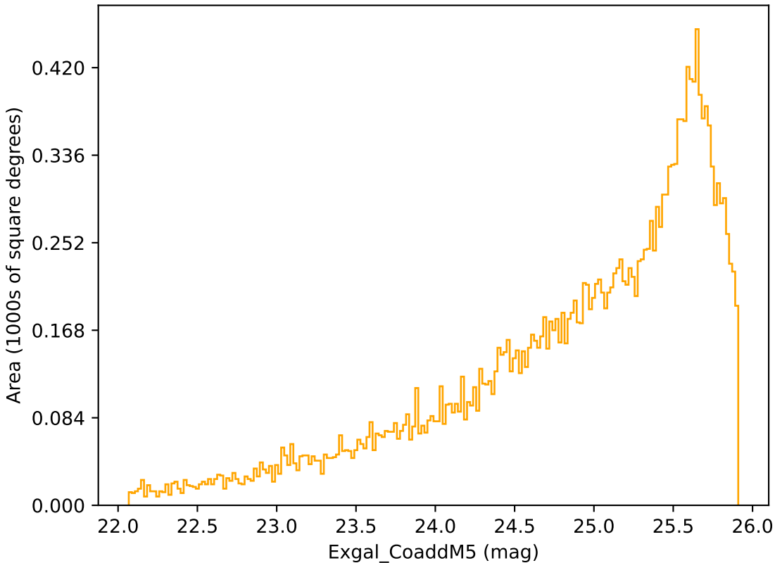
too_100_1v3.4_10yrs Yr 3-4 r band: Exgal_CoaddM5
