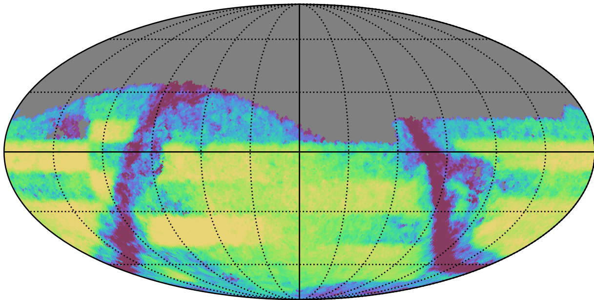
too_100_1v3.4_10yrs Yr 3-4 i band: Exgal_CoaddM5
