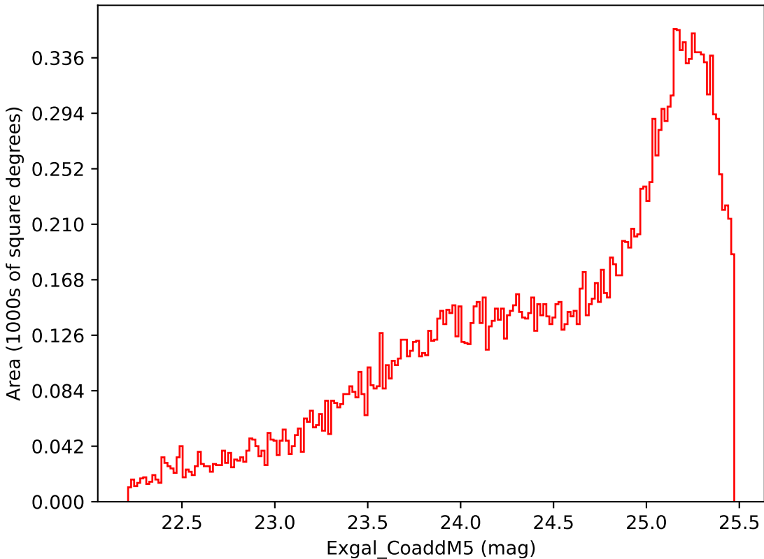
too_100_1v3.4_10yrs Yr 3-4 i band: Exgal_CoaddM5
