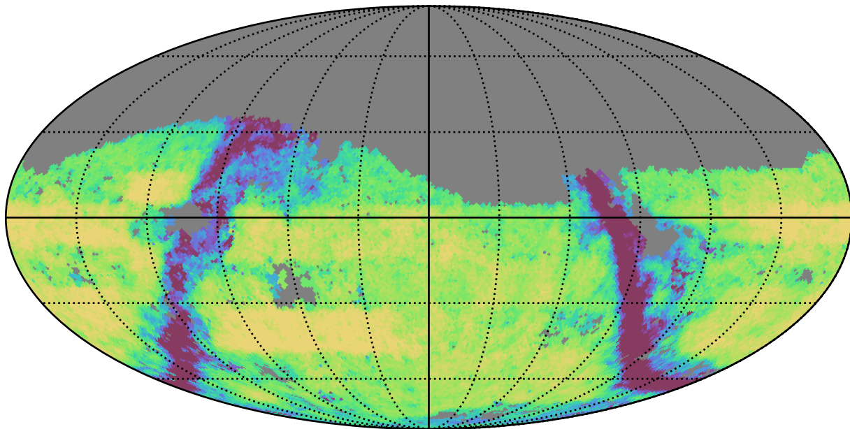
too_100_1v3.4_10yrs Yr 3-4 g band: Exgal_CoaddM5
