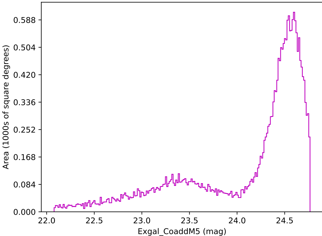
too_100_1v3.4_10yrs Yr 1 z band: Exgal_CoaddM5
