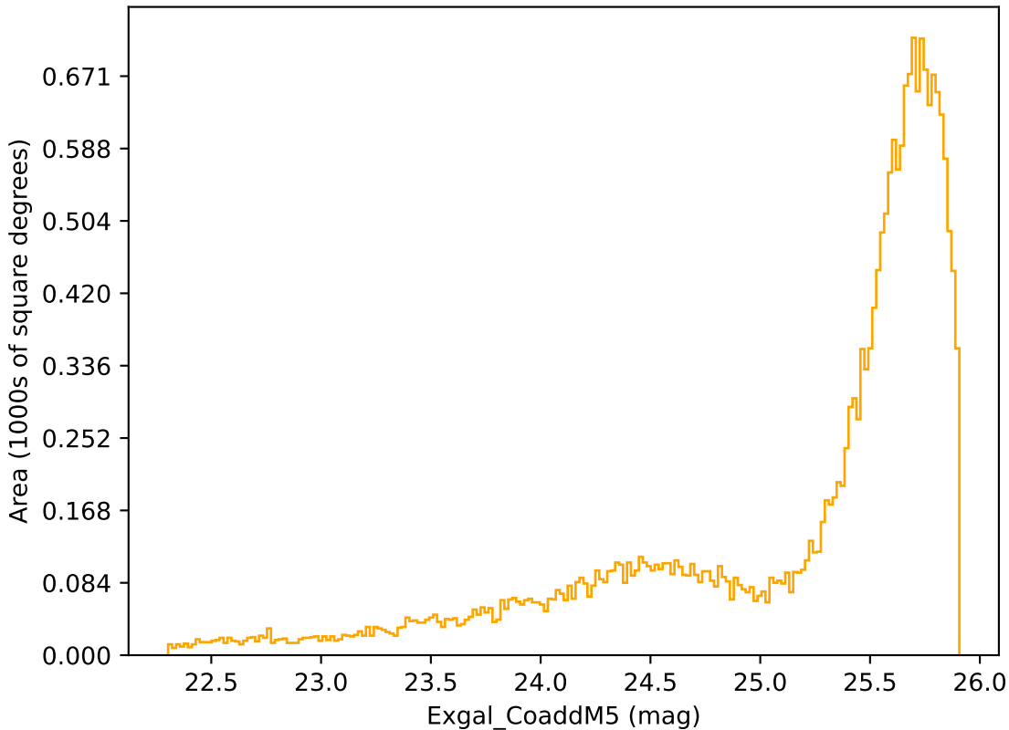
too_100_1v3.4_10yrs Yr 1 r band: Exgal_CoaddM5
