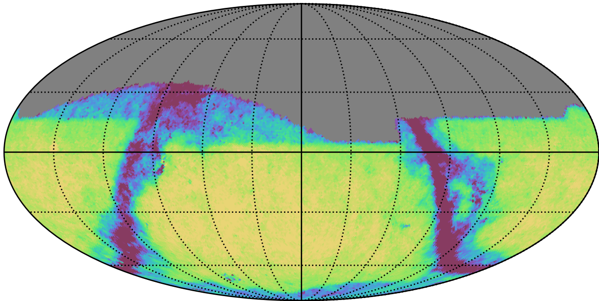
too_100_1v3.4_10yrs Yr 1 i band: Exgal_CoaddM5
