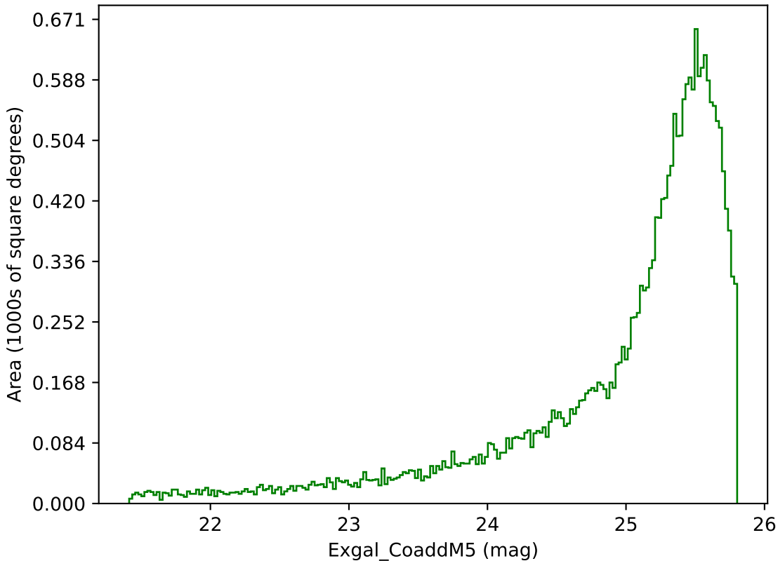
too_100_1v3.4_10yrs Yr 1 g band: Exgal_CoaddM5
