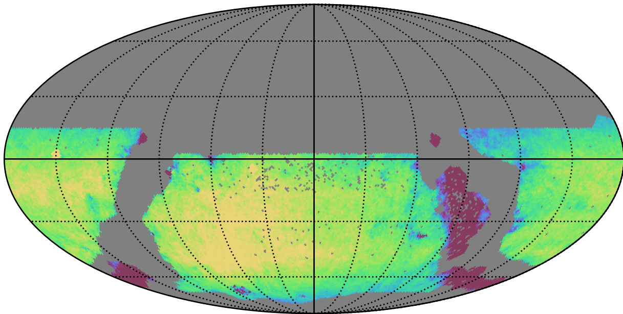
too_100_1v3.4_10yrs WFD z band: Exgal_CoaddM5
