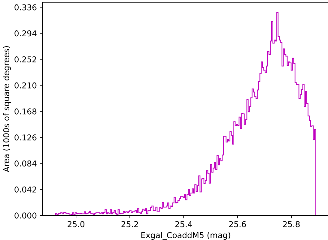
too_100_1v3.4_10yrs WFD z band: Exgal_CoaddM5
