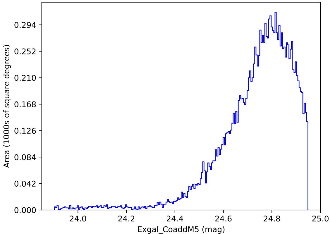
too_100_1v3.4_10yrs WFD y band: Exgal_CoaddM5
