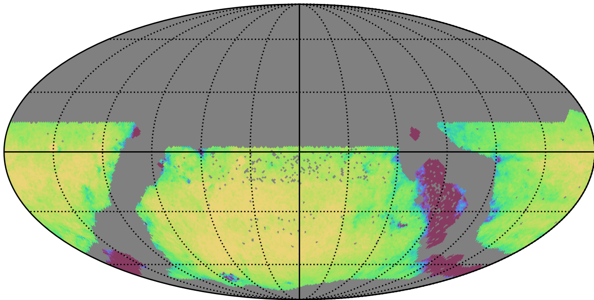
too_100_1v3.4_10yrs WFD u band: Exgal_CoaddM5
