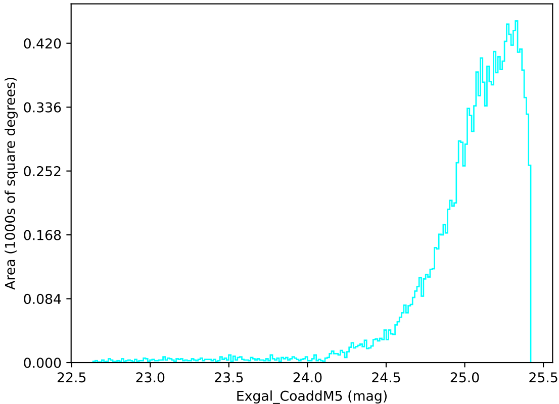
too_100_1v3.4_10yrs WFD u band: Exgal_CoaddM5
