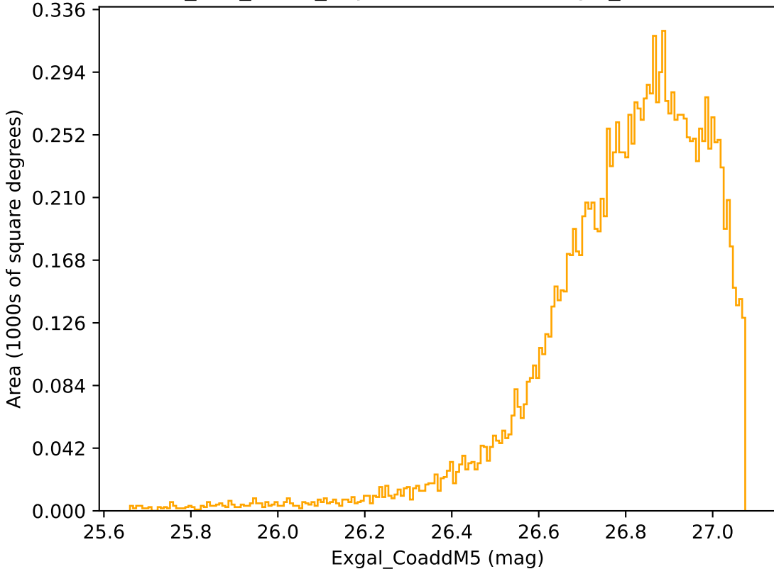
too_100_1v3.4_10yrs WFD r band: Exgal_CoaddM5
