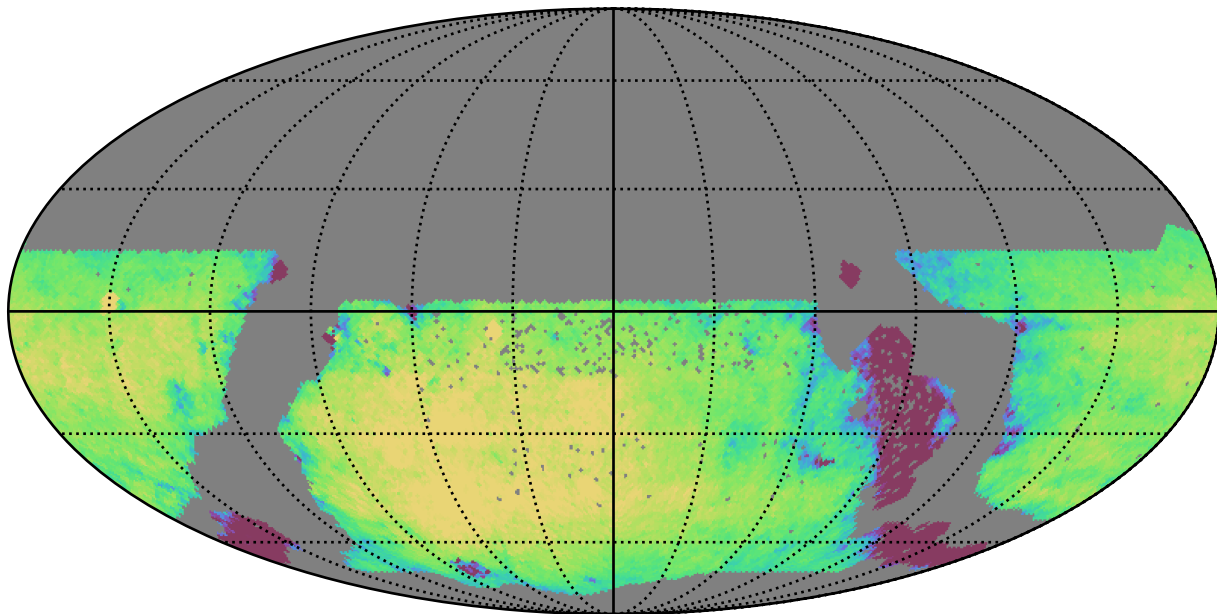
too_100_1v3.4_10yrs WFD g band: Exgal_CoaddM5
