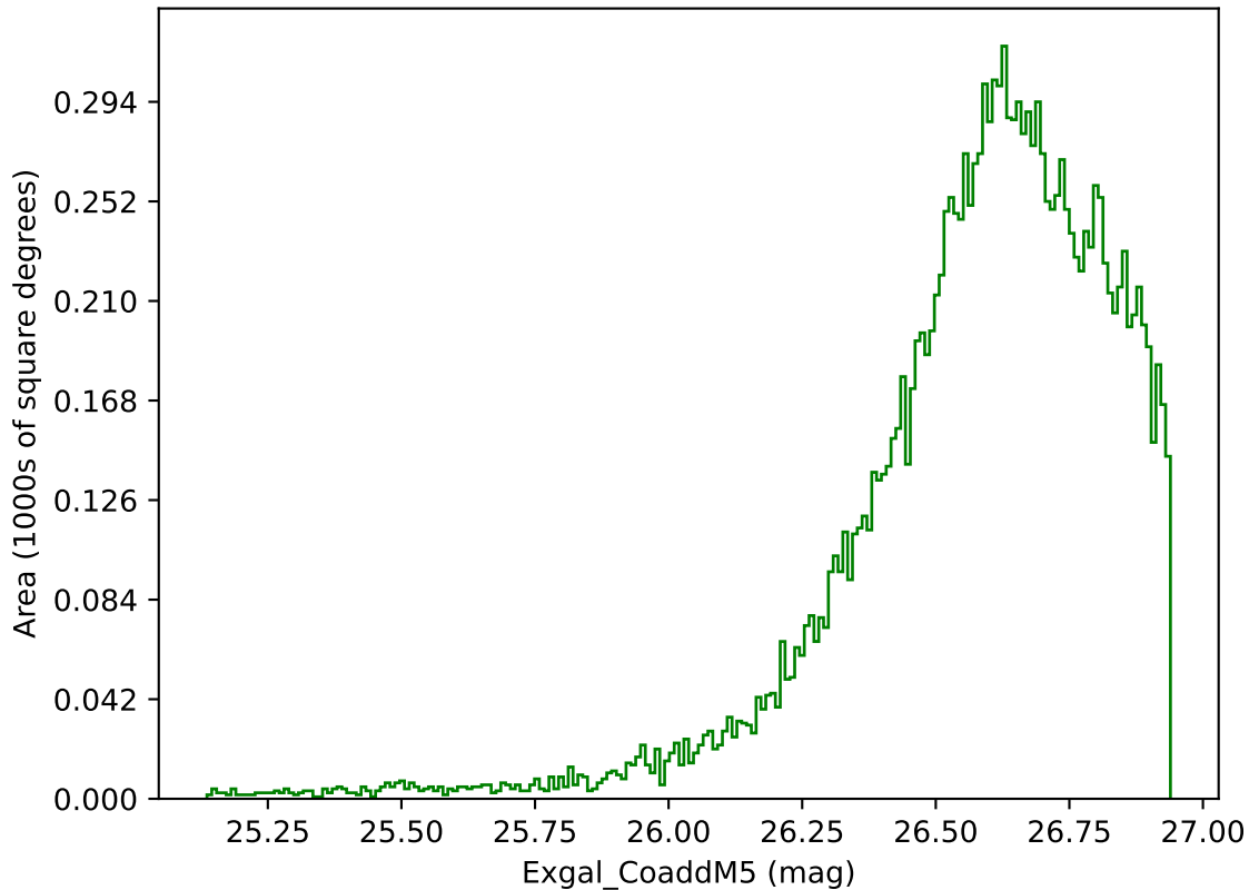
too_100_1v3.4_10yrs WFD g band: Exgal_CoaddM5
