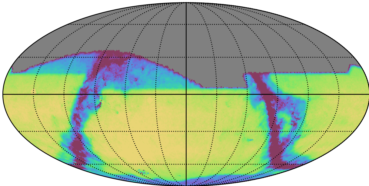
too_100_1v3.4_10yrs All sky z band: Exgal_CoaddM5
