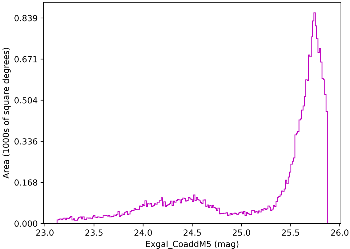
too_100_1v3.4_10yrs All sky z band: Exgal_CoaddM5
