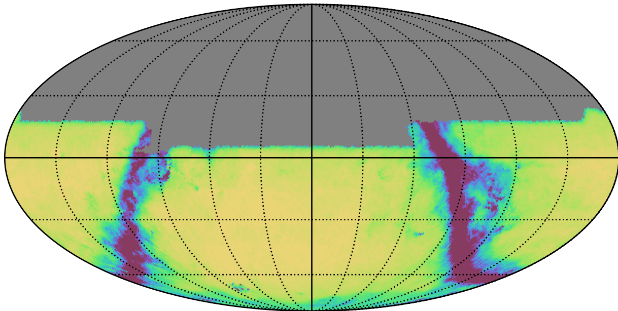
too_100_1v3.4_10yrs All sky u band: Exgal_CoaddM5
