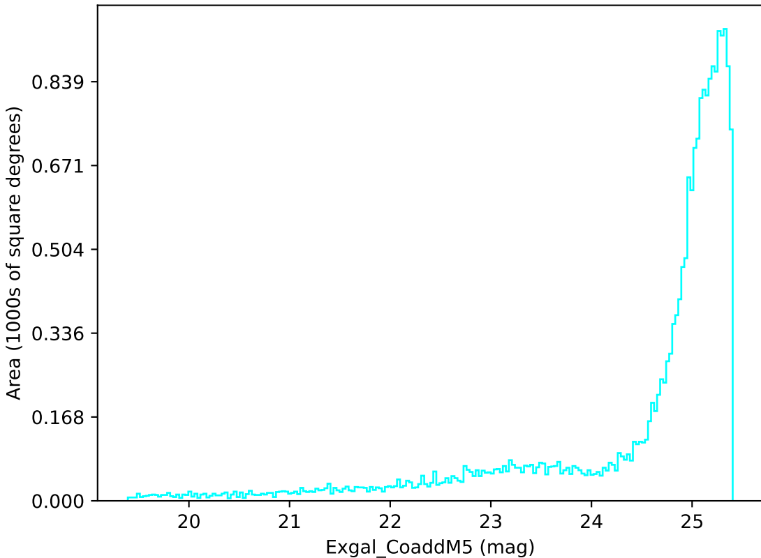
too_100_1v3.4_10yrs All sky u band: Exgal_CoaddM5
